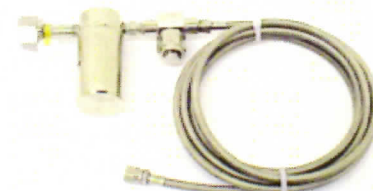
LCO 2 Filter Housing (#8784) installed onto High Pressure Hose
